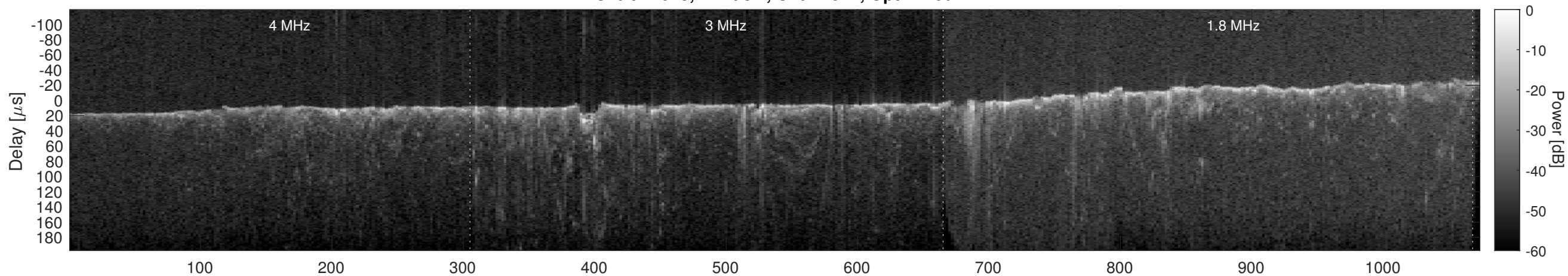
Orbit 17628, Cluttergram
