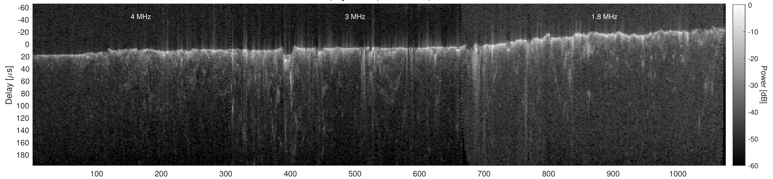
Orbit 17628, Cluttergram
