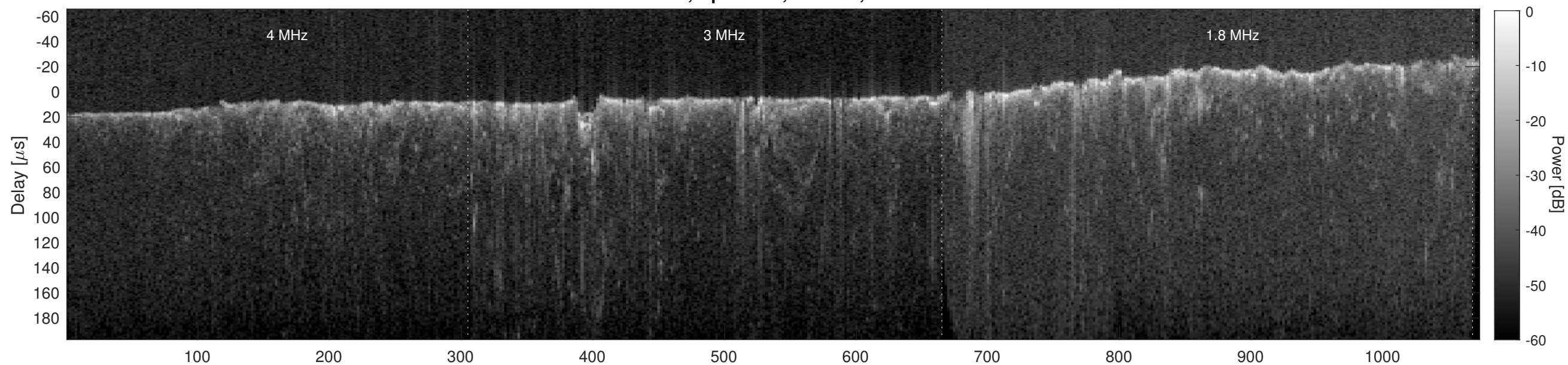
Orbit 17628, Cluttergram
