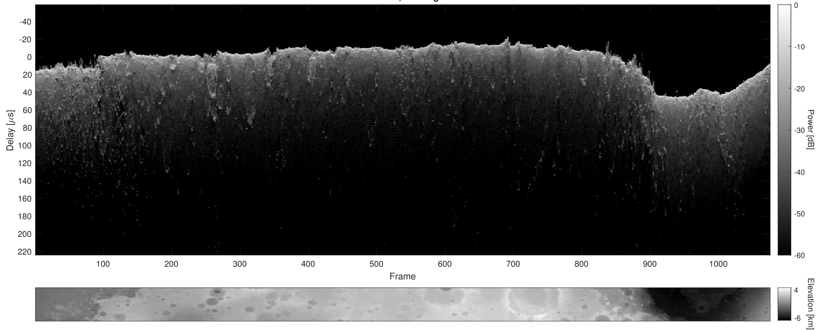
Orbit 17631, Cluttergram
