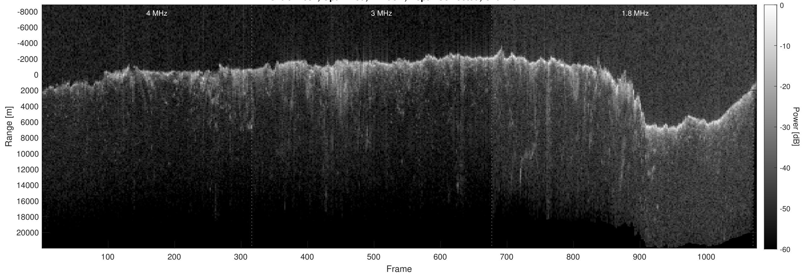
Orbit 17631, Optimized, Window, Depth-Corrected, Channel 2
