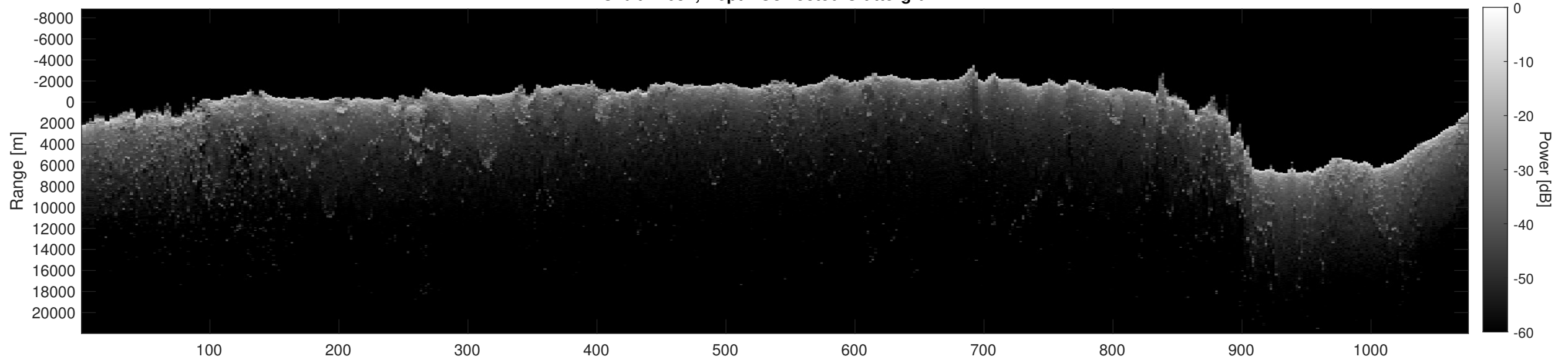
Orbit 17631, Depth-Corrected Cluttergram
