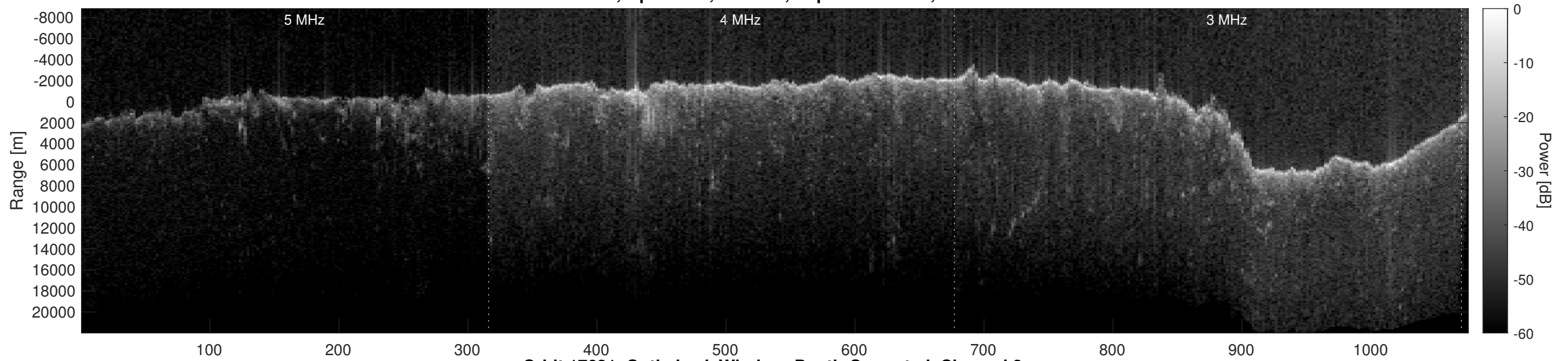
Orbit 17631, Optimized, Window, Depth-Corrected, Channel 2
