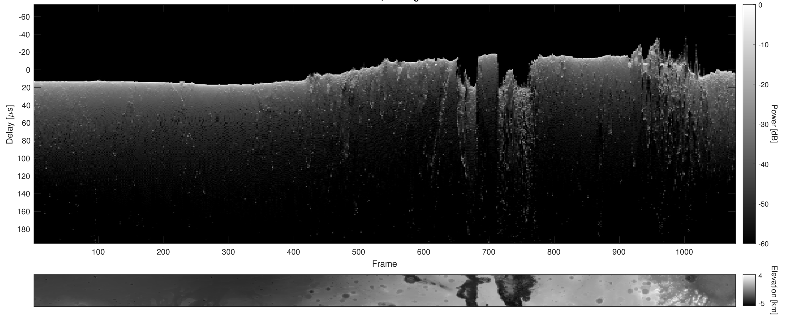
Orbit 17632, Cluttergram
