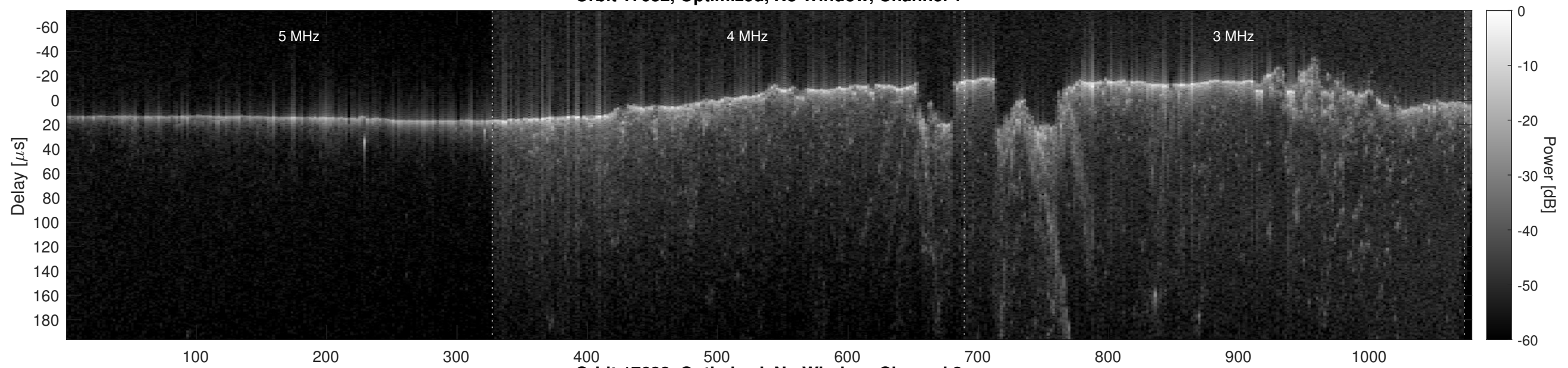
Orbit 17632, Optimized, No Window, Channel 2
