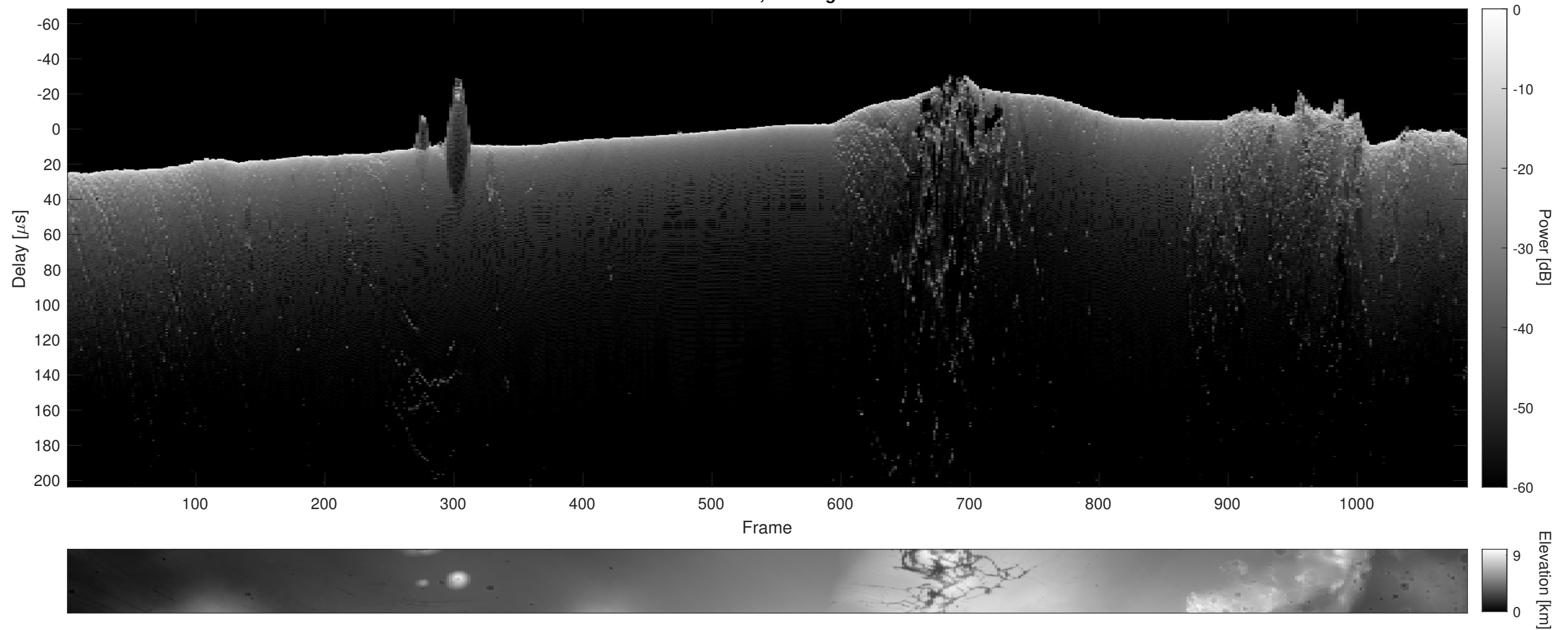
Orbit 17636, Cluttergram
