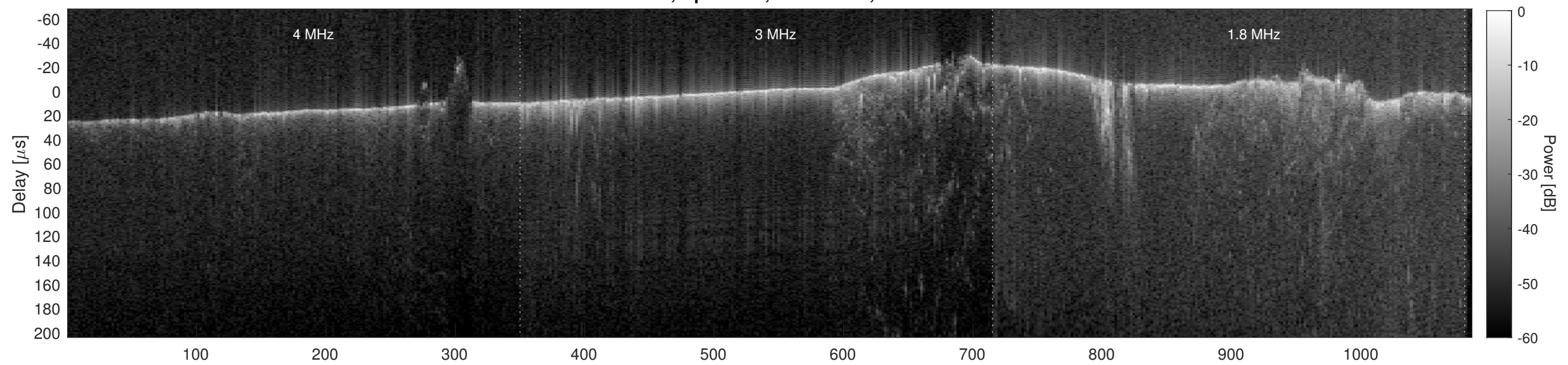
Orbit 17636, Cluttergram
