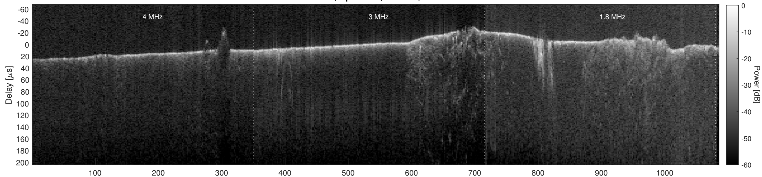
Orbit 17636, Cluttergram
