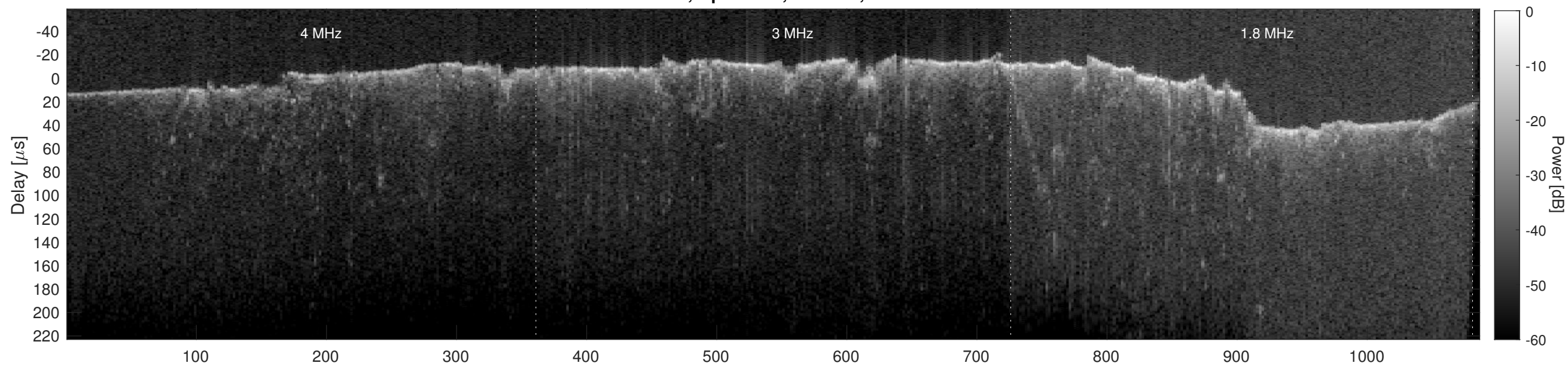
Orbit 17638, Cluttergram
