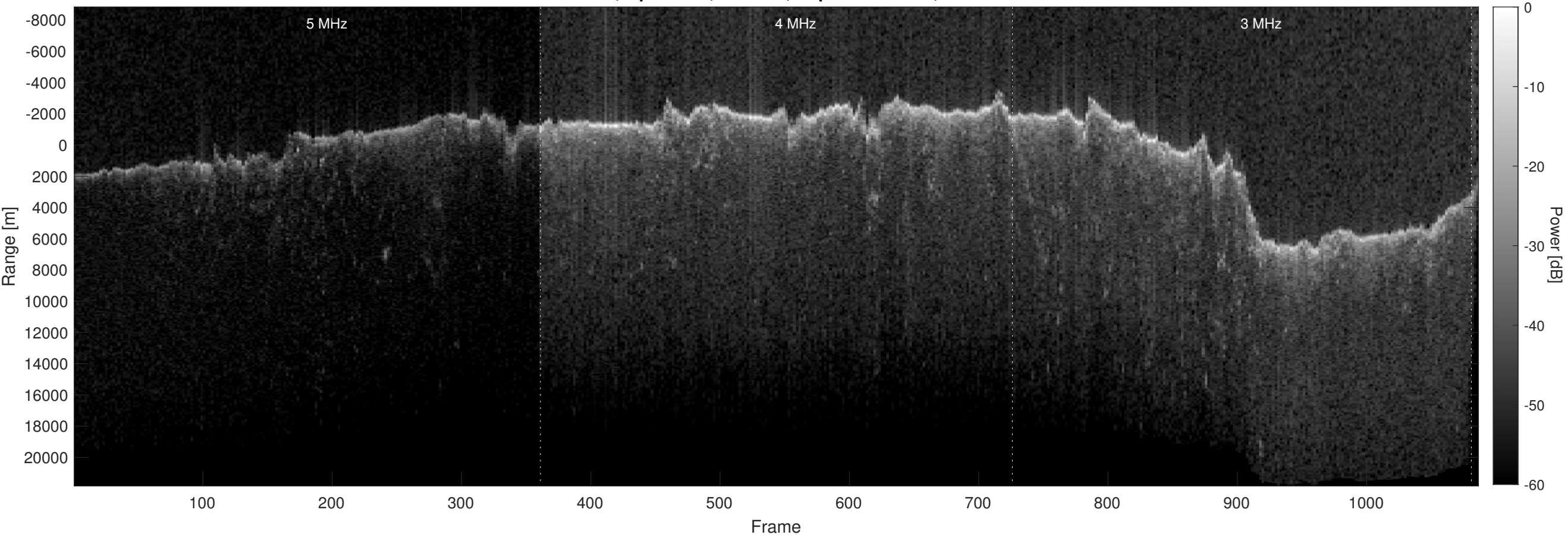
Orbit 17638, Optimized, Window, Depth-Corrected, Channel 2
