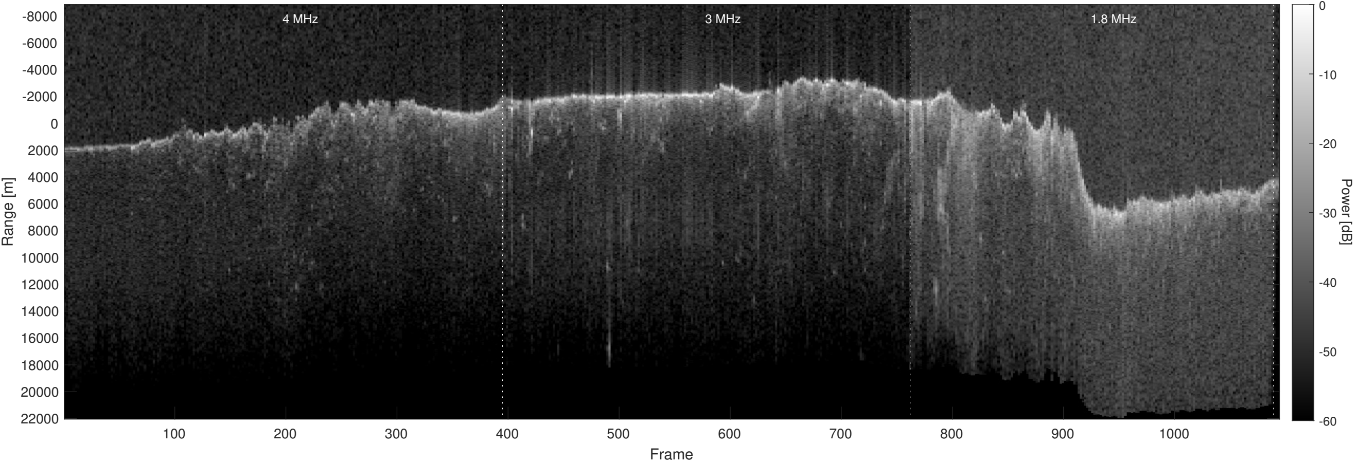
Orbit 17645, Optimized, Window, Depth-Corrected, Channel 2
