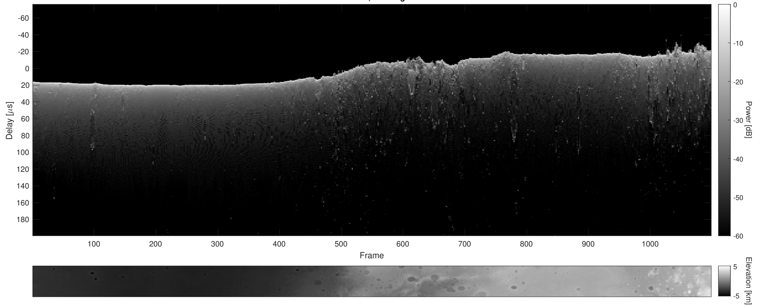
Orbit 17648, Cluttergram
