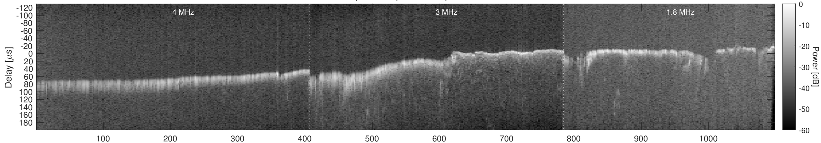
Orbit 17648, Window, Channel 2, Chapman
