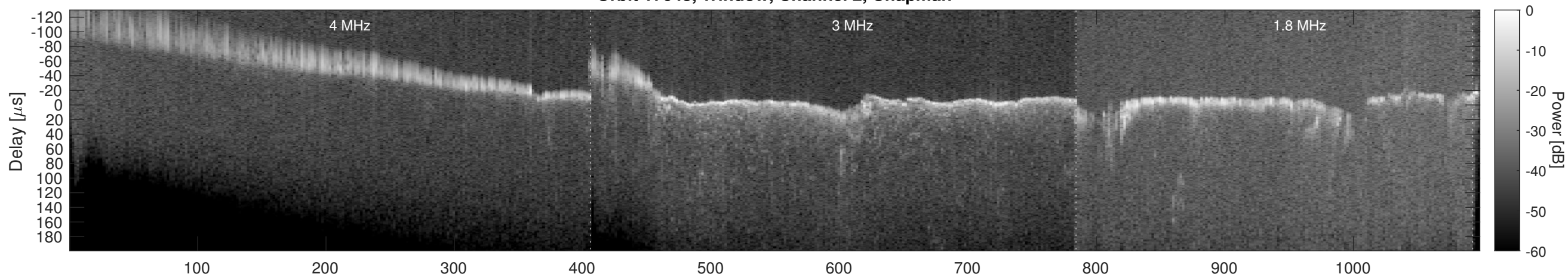
Orbit 17648, Window, Channel 2, Optimized
