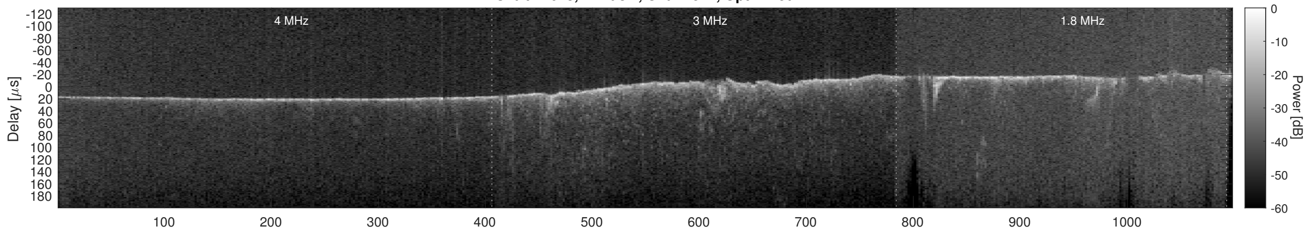
Orbit 17648, Cluttergram
