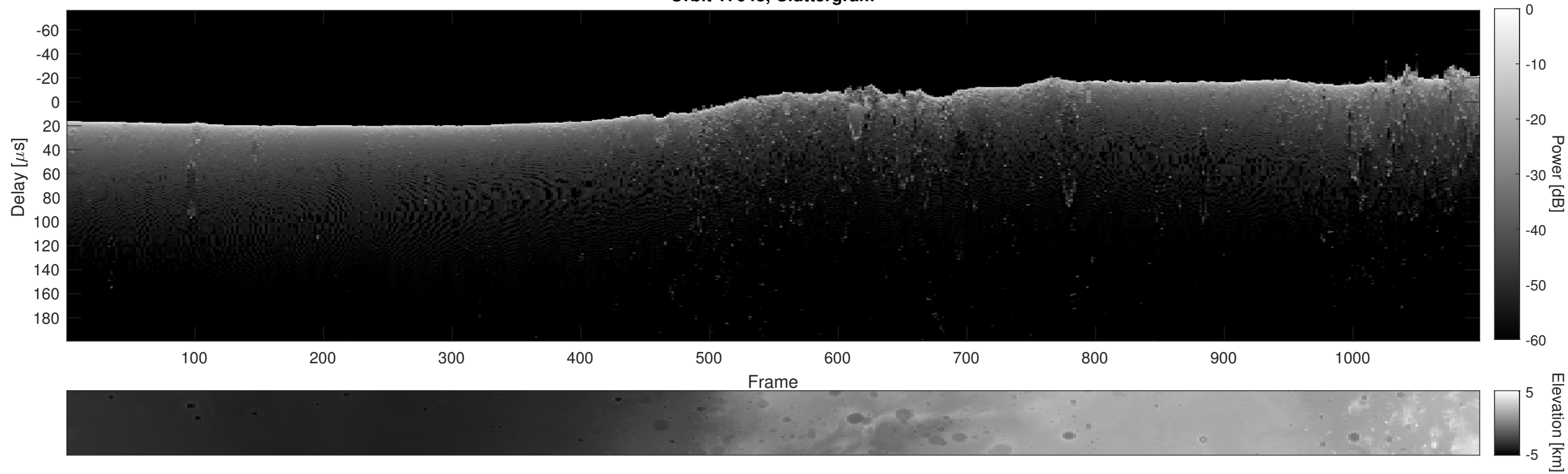
Orbit 17648, Cluttergram
