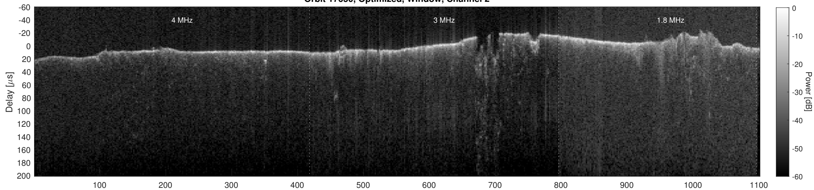
Orbit 17650, Cluttergram
