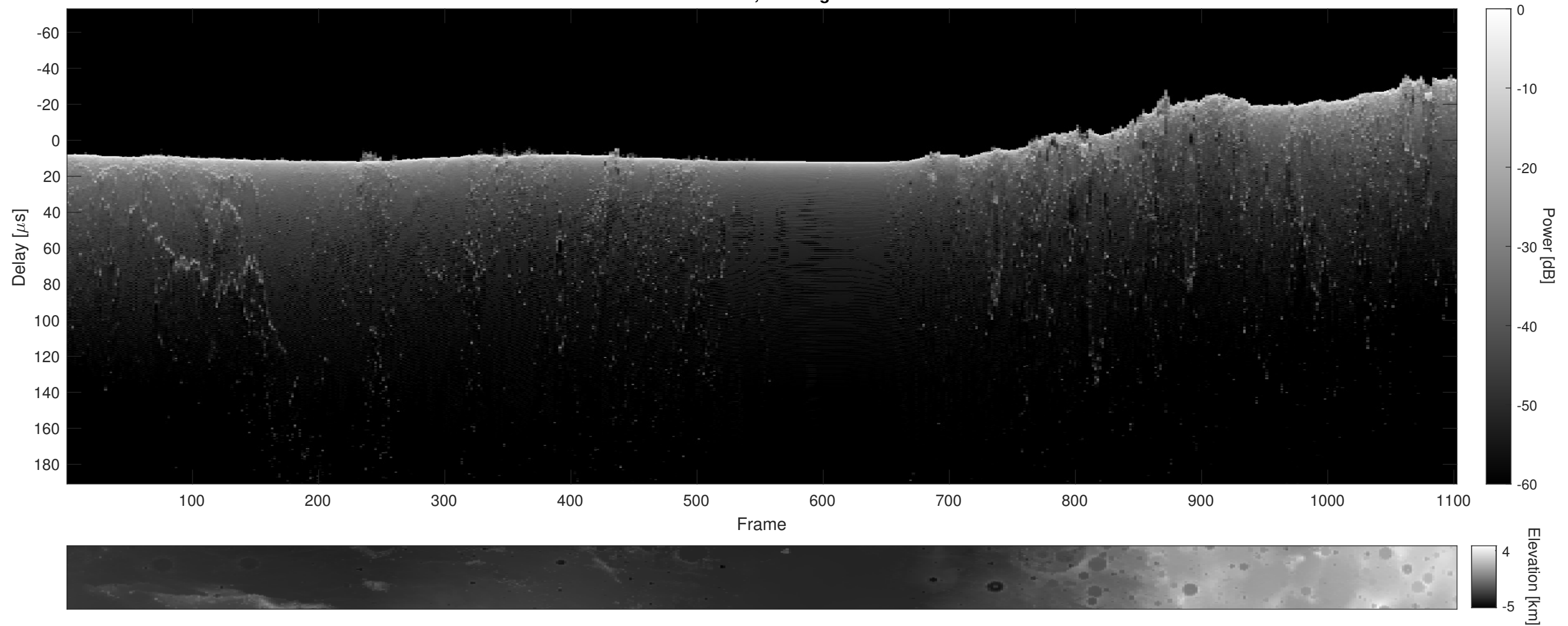
Orbit 17651, Cluttergram
