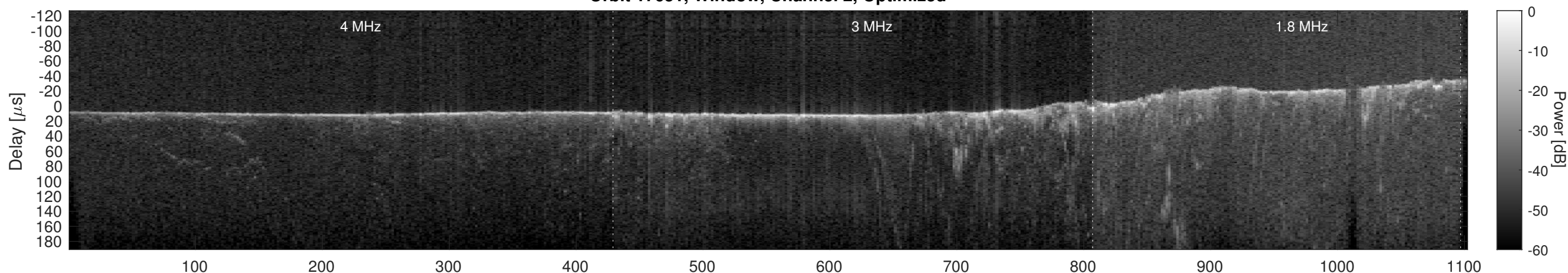
Orbit 17651, Cluttergram
