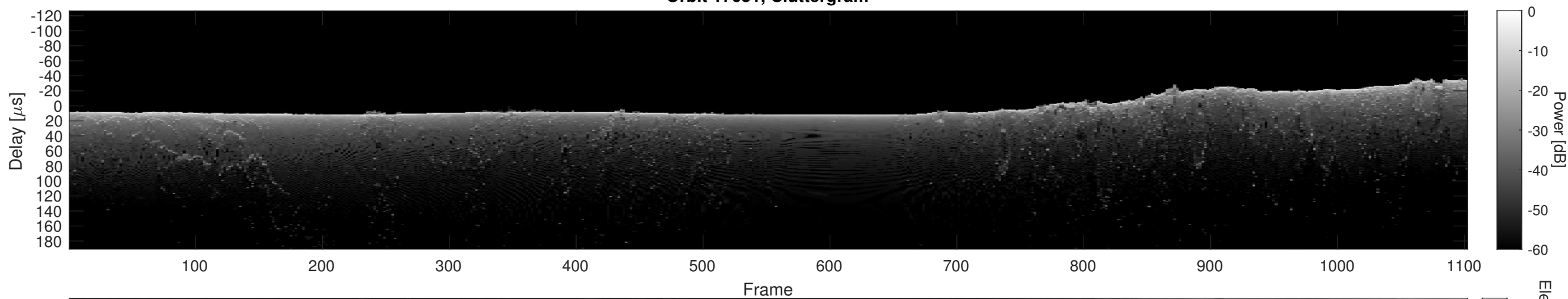
Orbit 17651, Cluttergram
