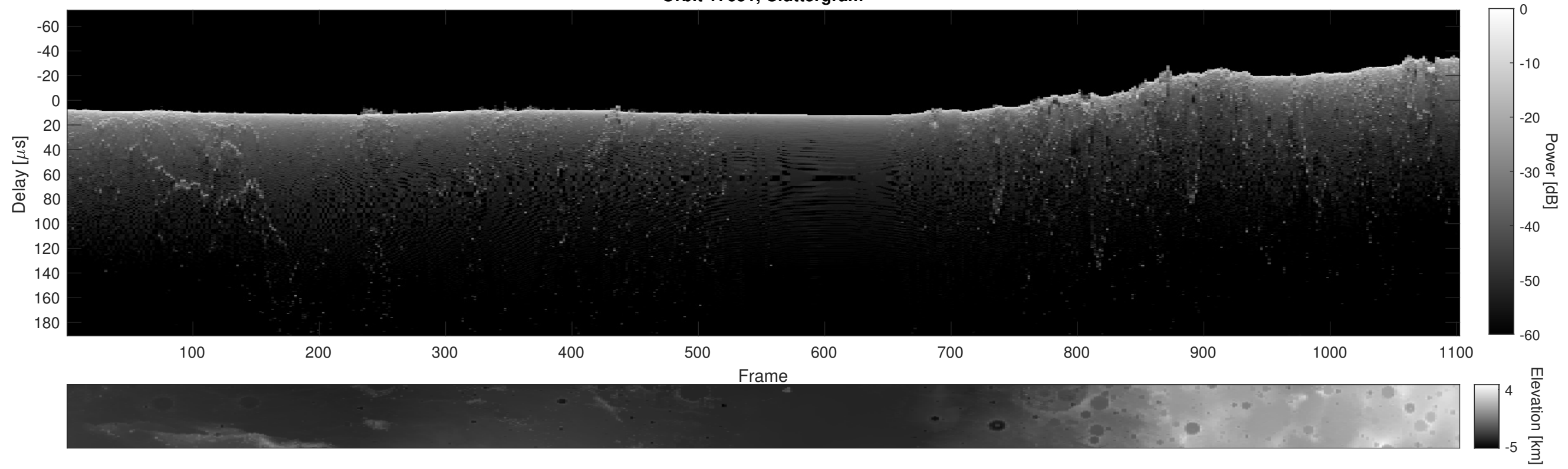
Orbit 17651, Cluttergram
