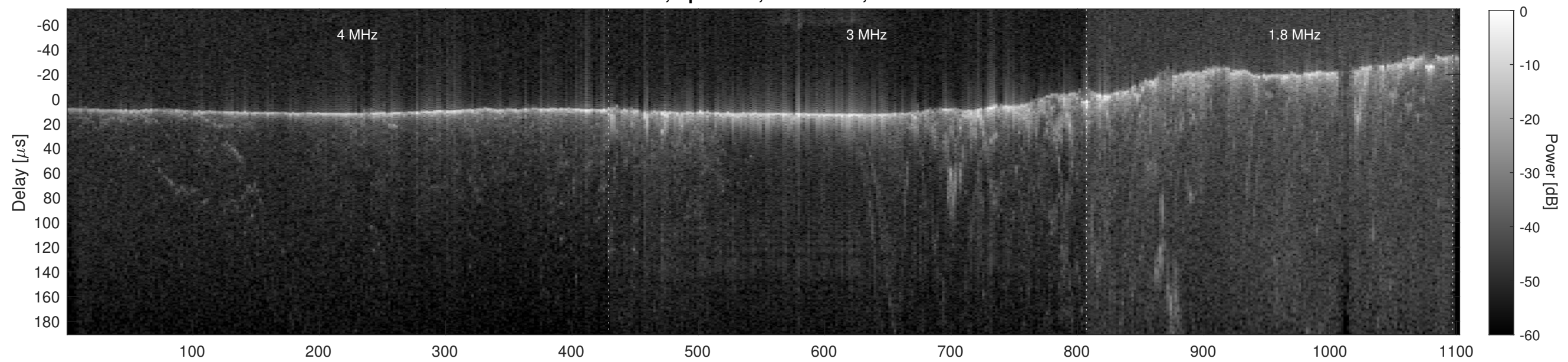
Orbit 17651, Cluttergram
