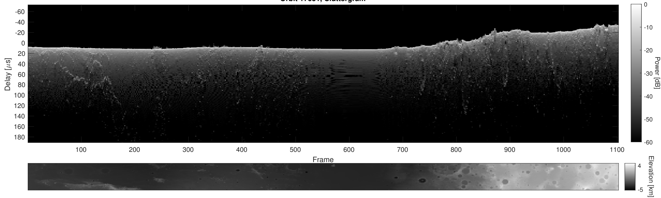
Orbit 17651, Cluttergram
