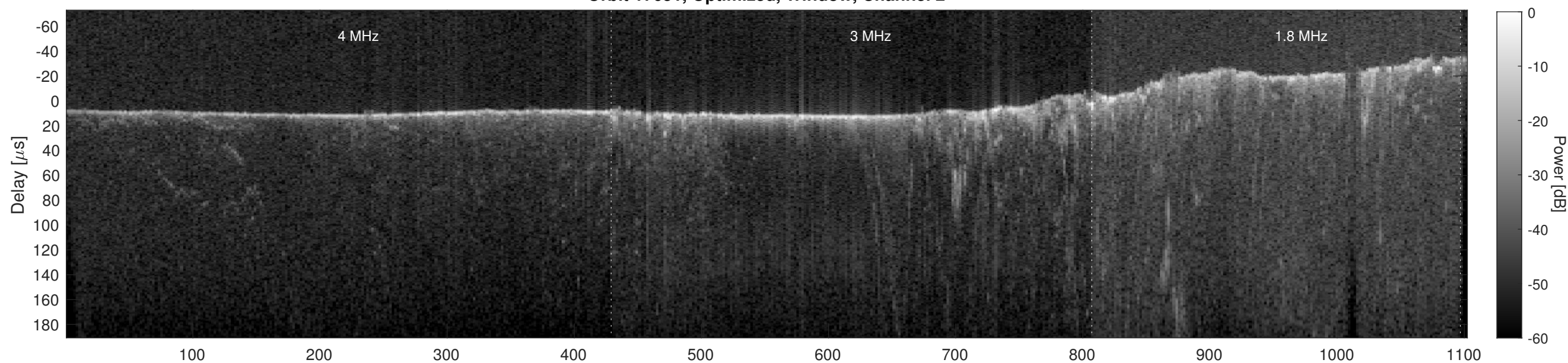
Orbit 17651, Cluttergram
