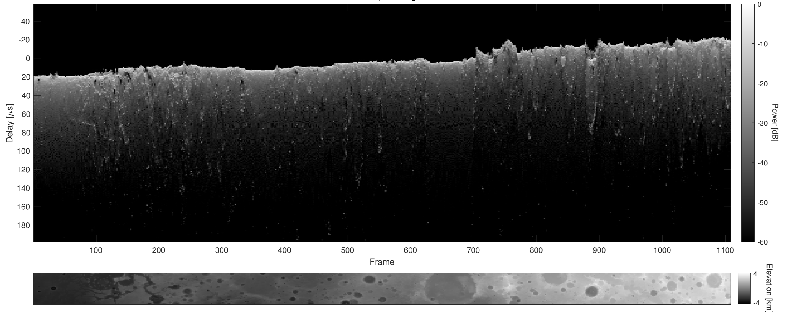
Orbit 17656, Cluttergram
