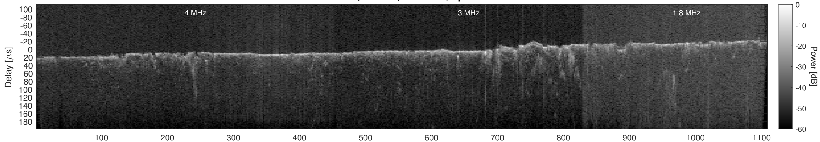
Orbit 17656, Cluttergram
