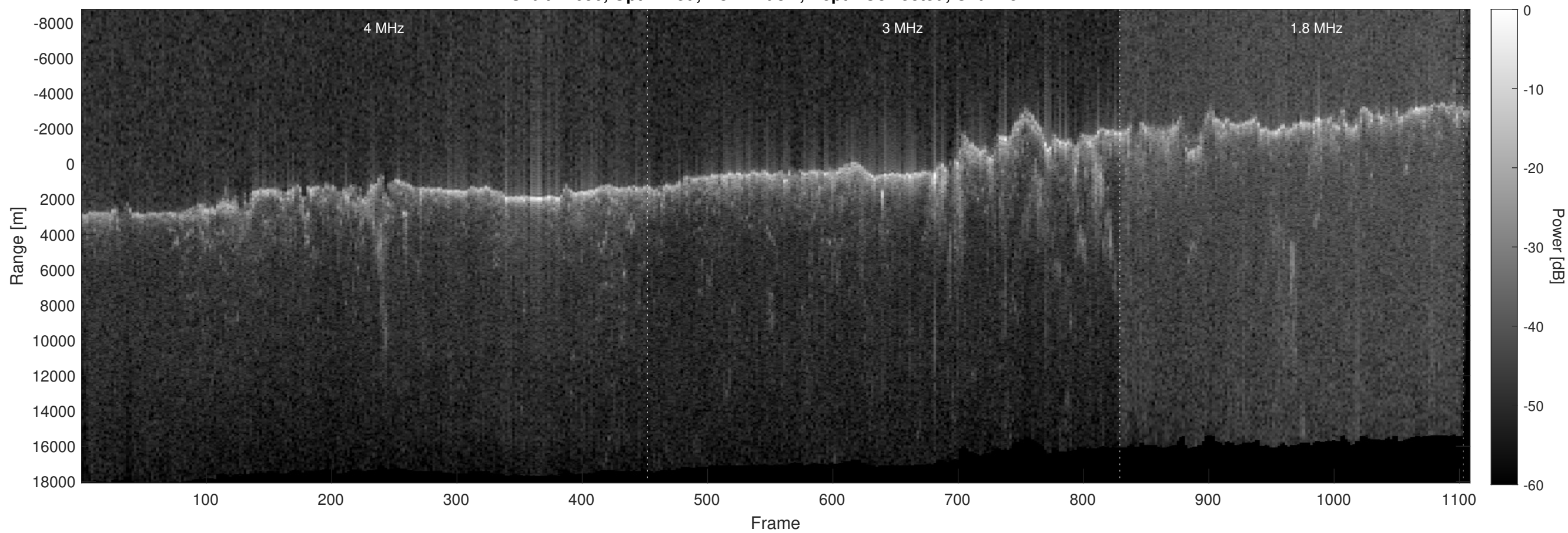
Orbit 17656, Optimized, No Window, Depth-Corrected, Channel 2
