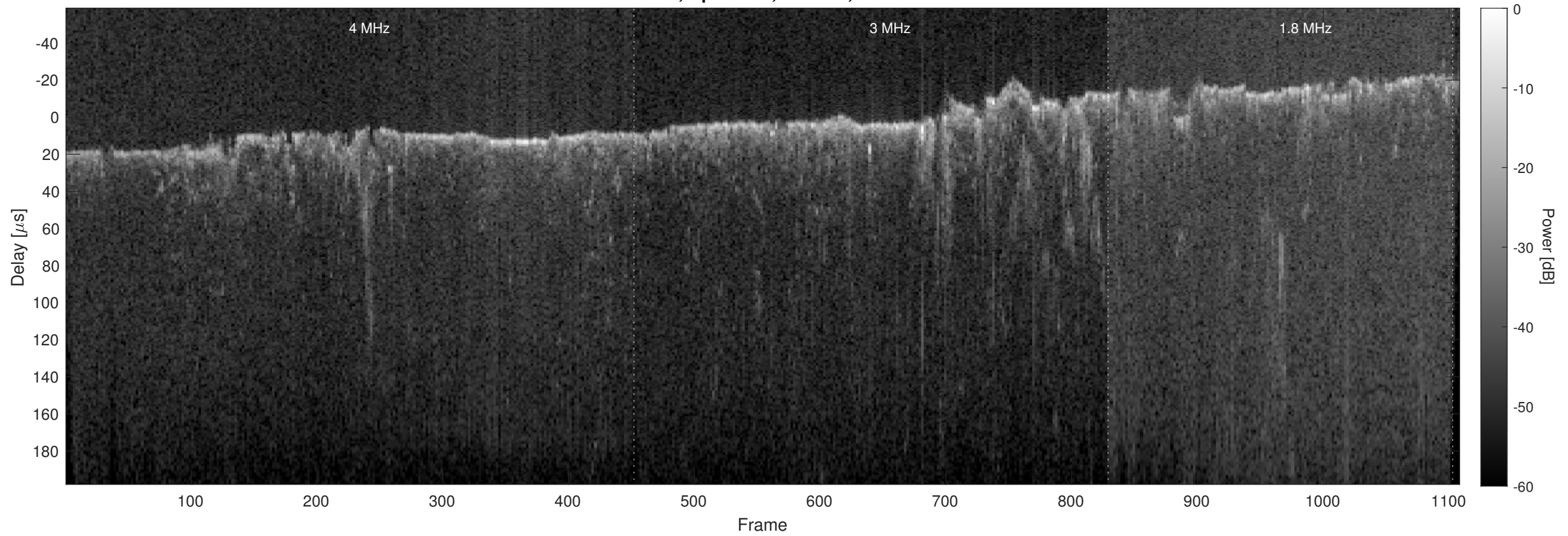
Orbit 17656, Optimized, Window, Channel 2
