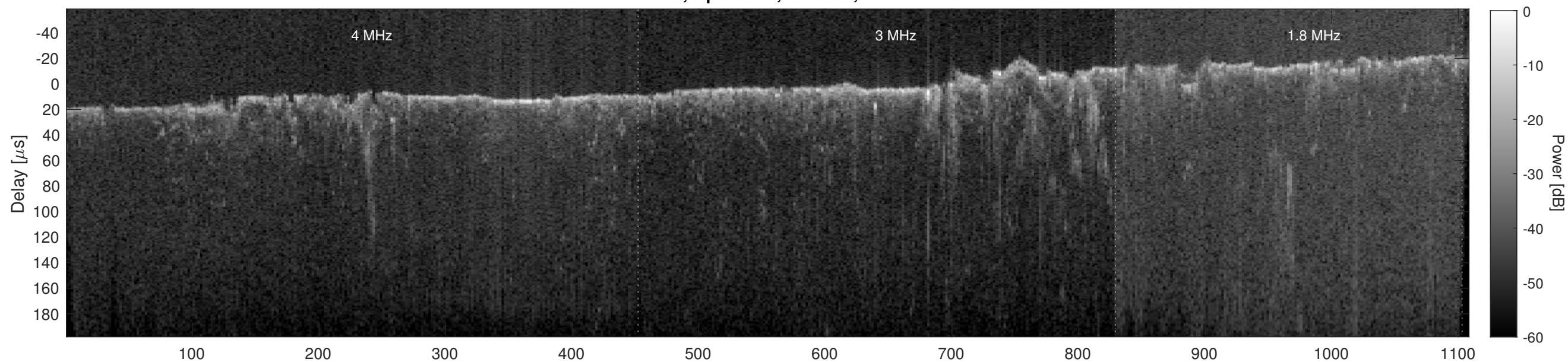
Orbit 17656, Cluttergram
