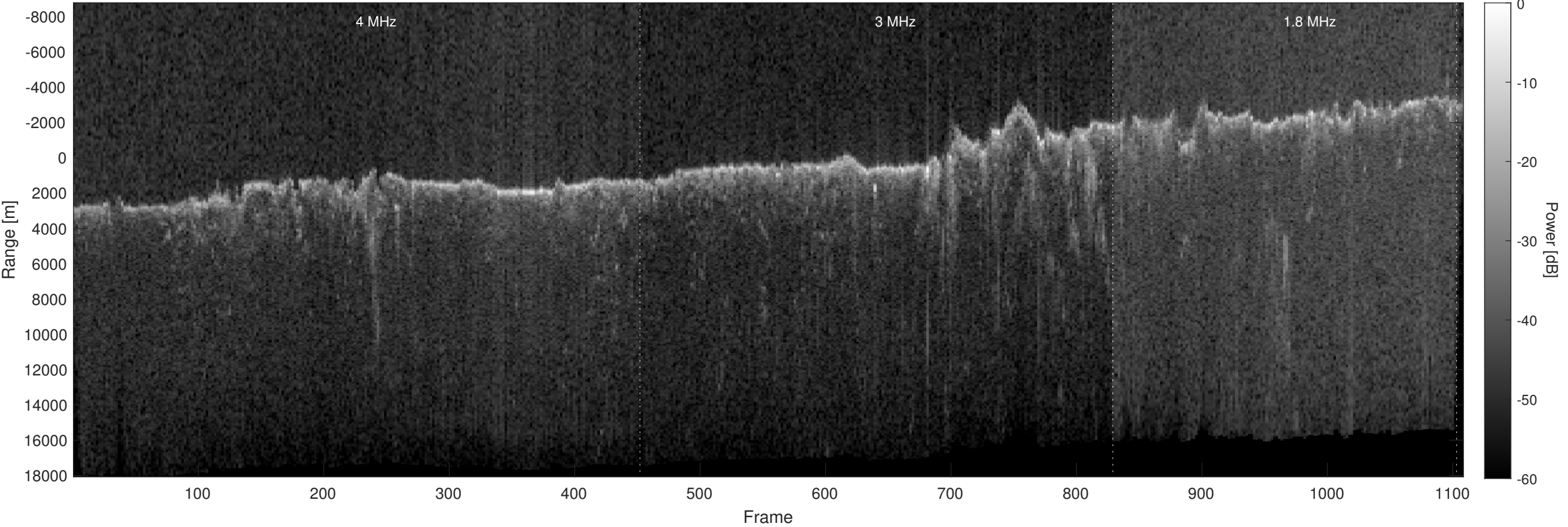
Orbit 17656, Optimized, Window, Depth-Corrected, Channel 2
