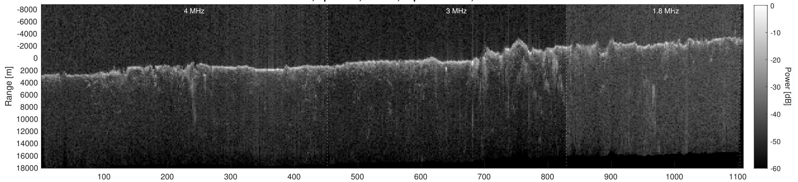
Orbit 17656, Depth-Corrected Cluttergram
