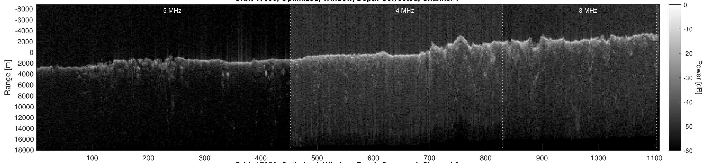
Orbit 17656, Optimized, Window, Depth-Corrected, Channel 2
