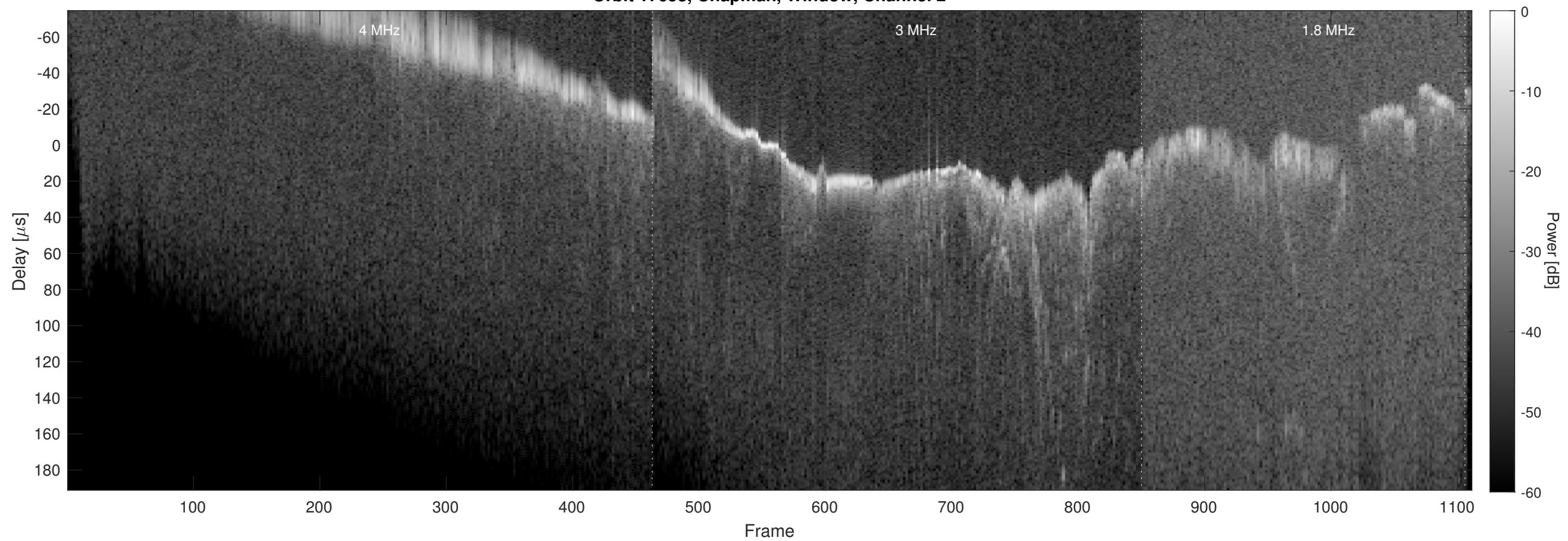
Orbit 17658, Chapman, Window, Channel 2
