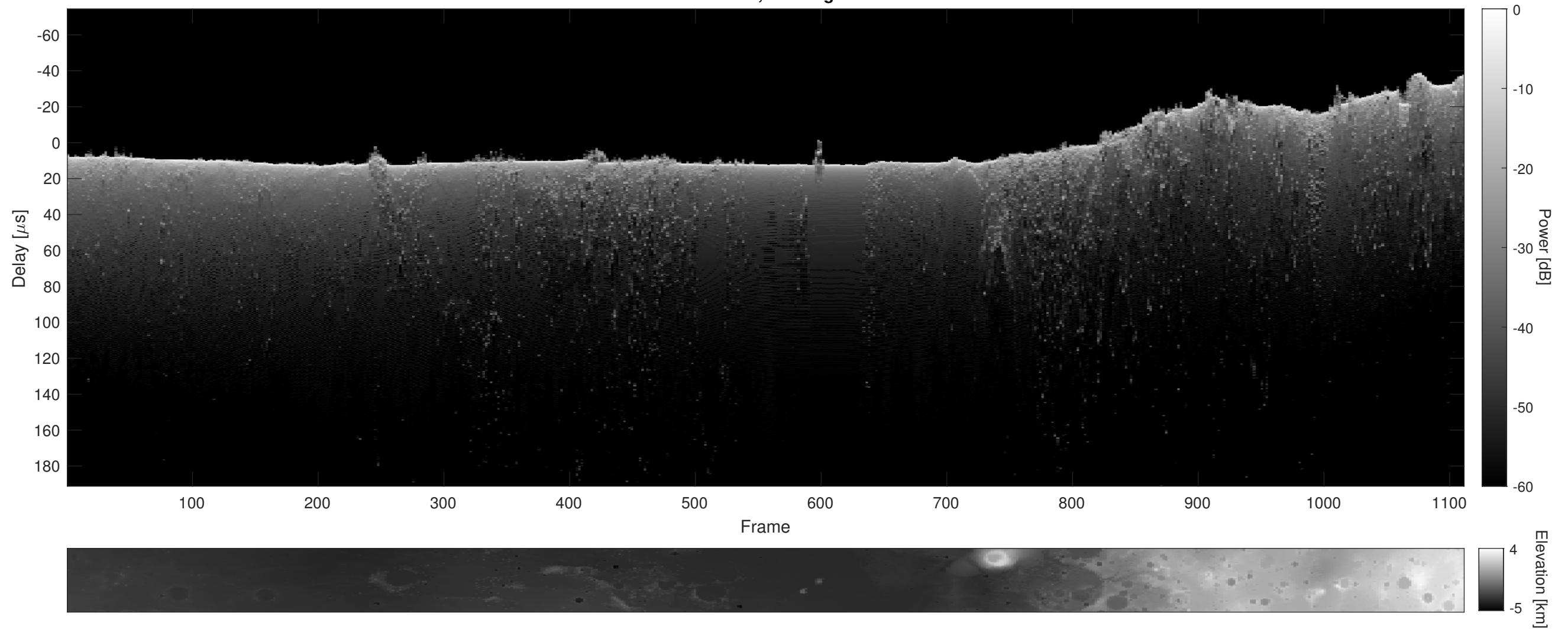
Orbit 17658, Cluttergram
