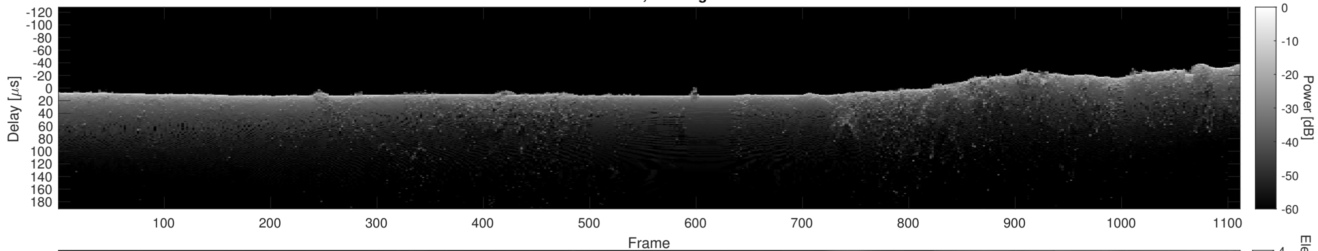
Orbit 17658, Cluttergram
