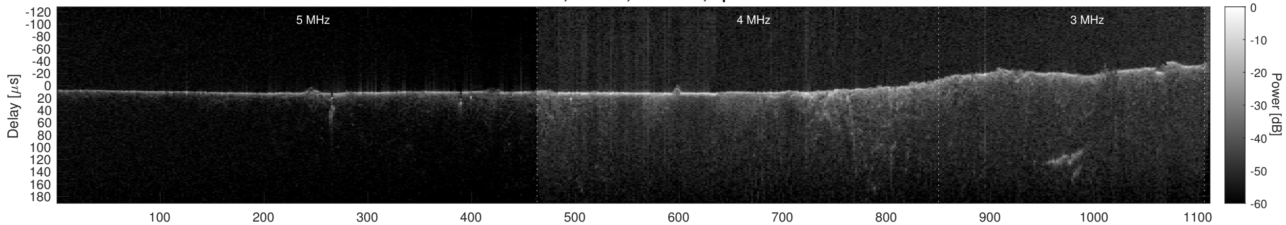
Orbit 17658, Cluttergram
