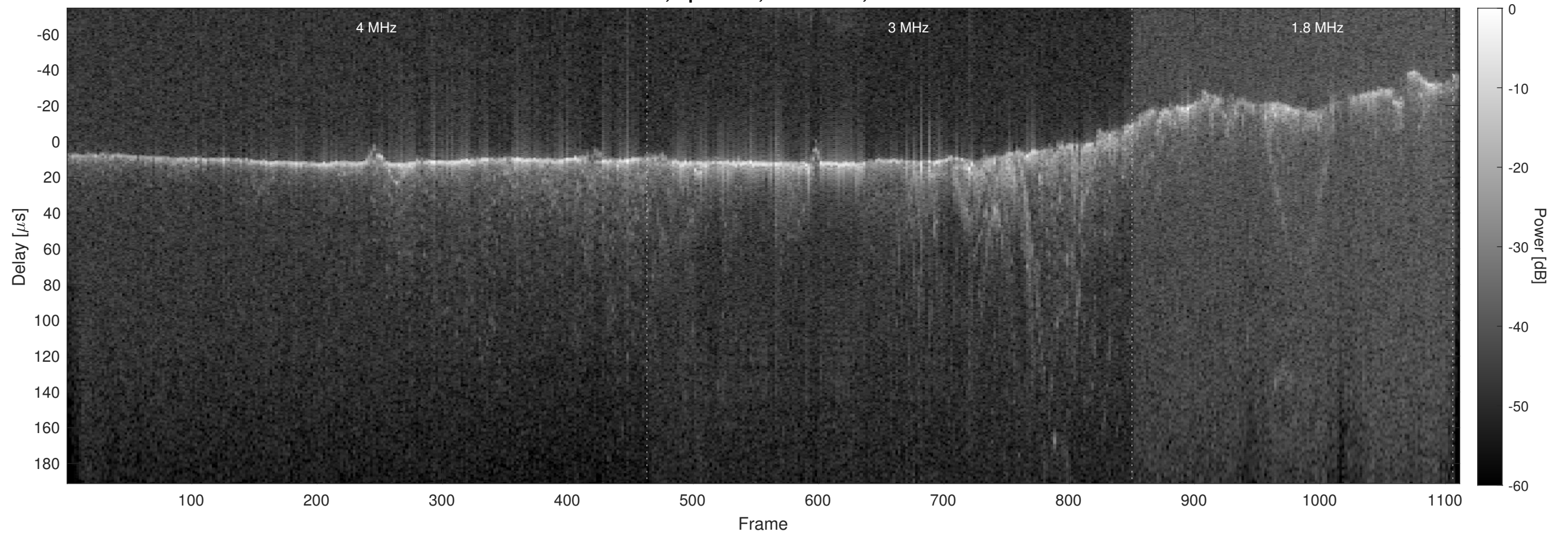
Orbit 17658, Optimized, No Window, Channel 2
