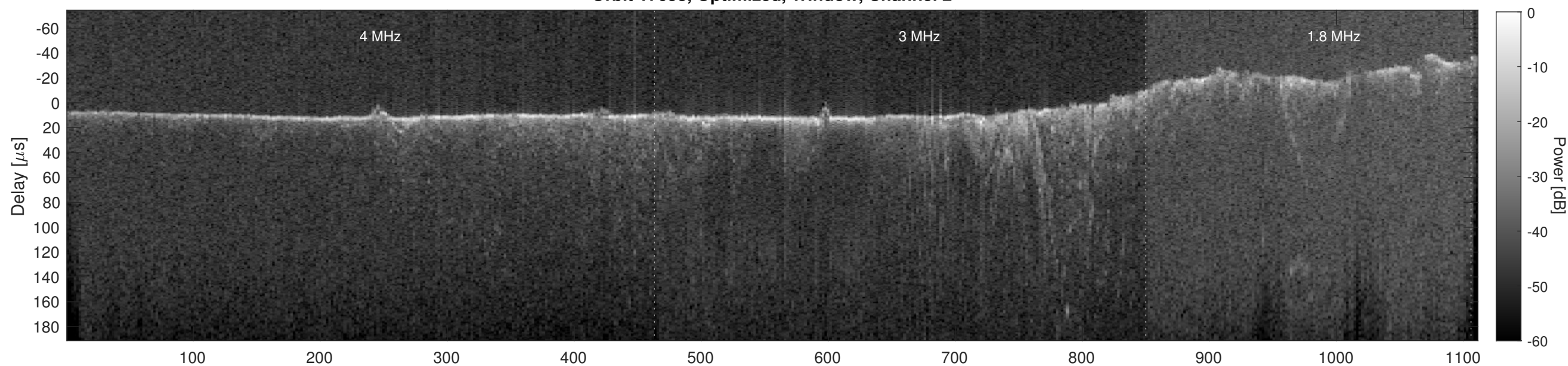
Orbit 17658, Cluttergram
