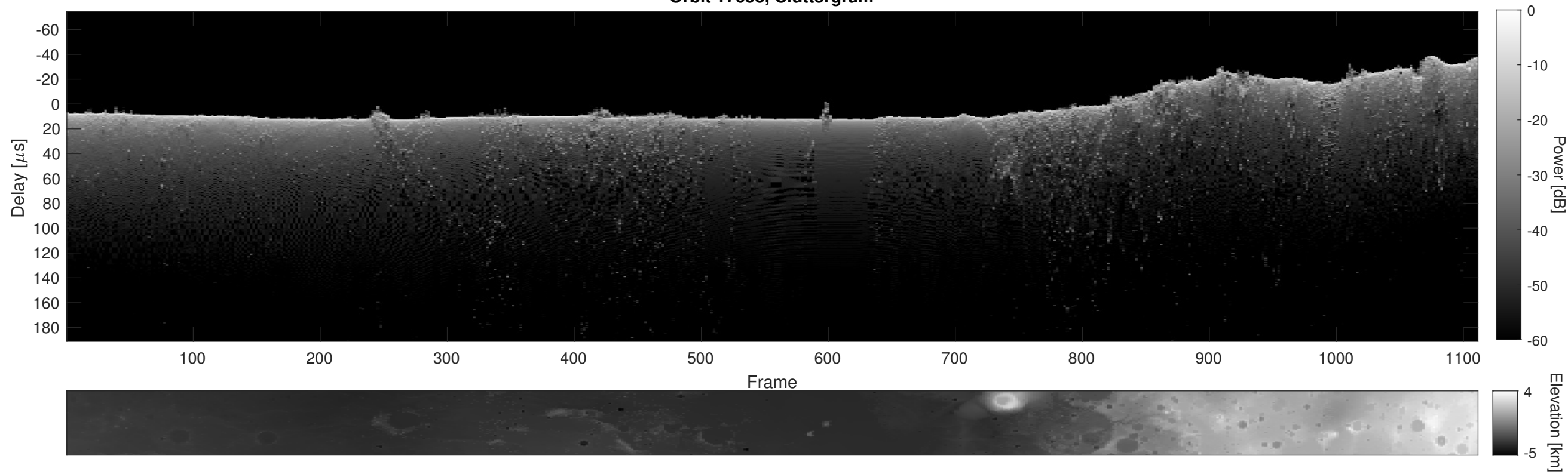
Orbit 17658, Cluttergram
