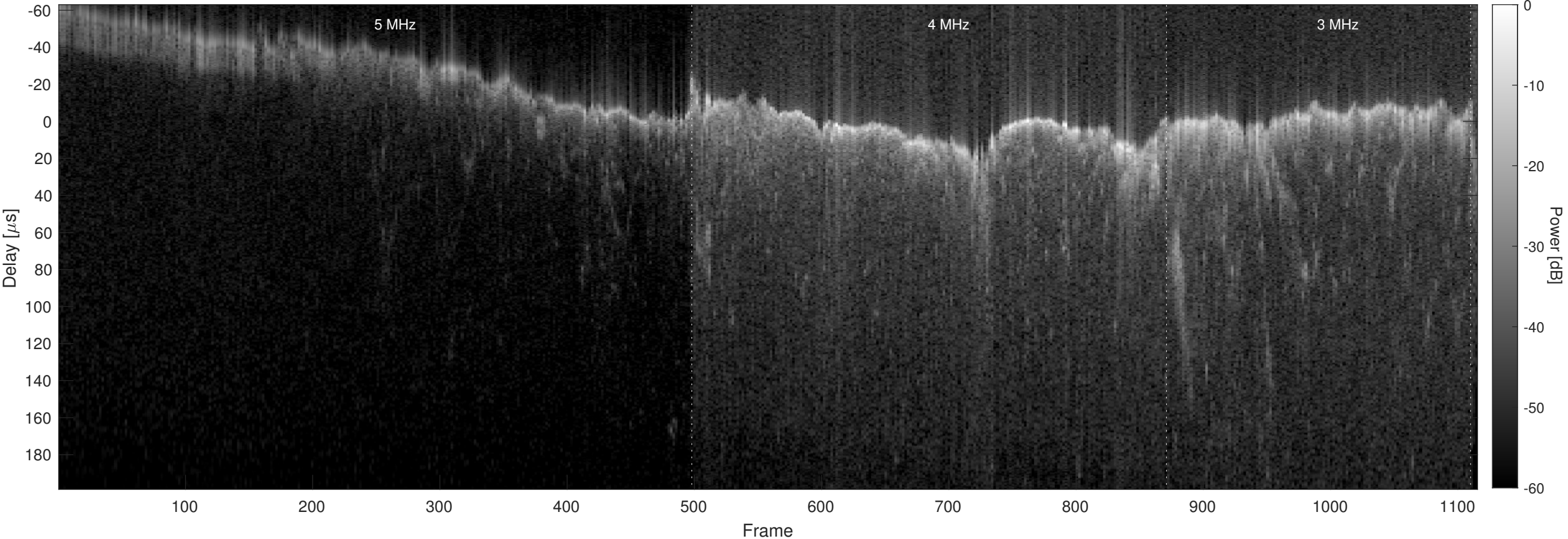
Orbit 17663, Chapman, No Window, Channel 2
