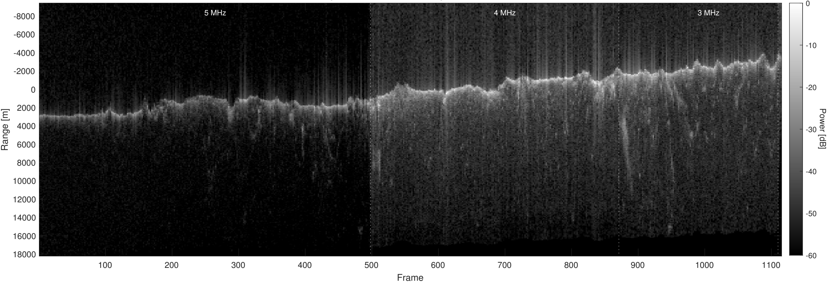
Orbit 17663, Optimized, No Window, Depth-Corrected, Channel 2
