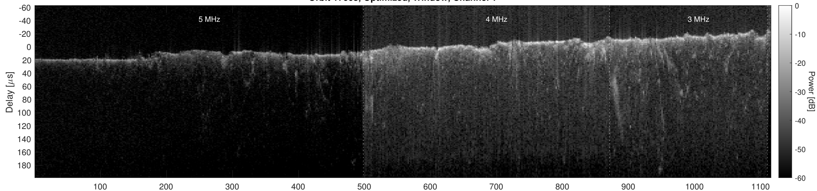
Orbit 17663, Optimized, Window, Channel 2
