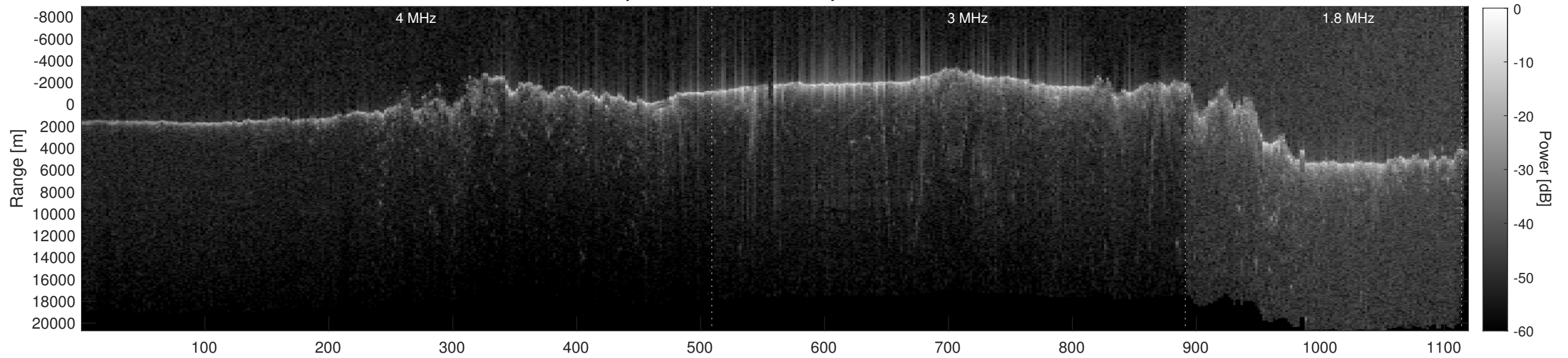
Orbit 17666, Depth-Corrected Cluttergram
