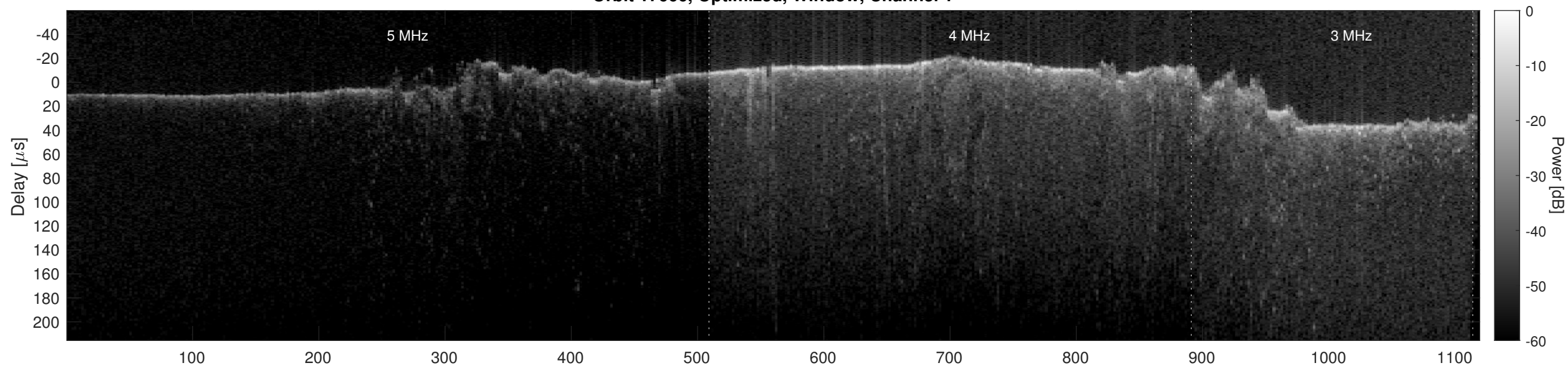
Orbit 17666, Optimized, Window, Channel 2
