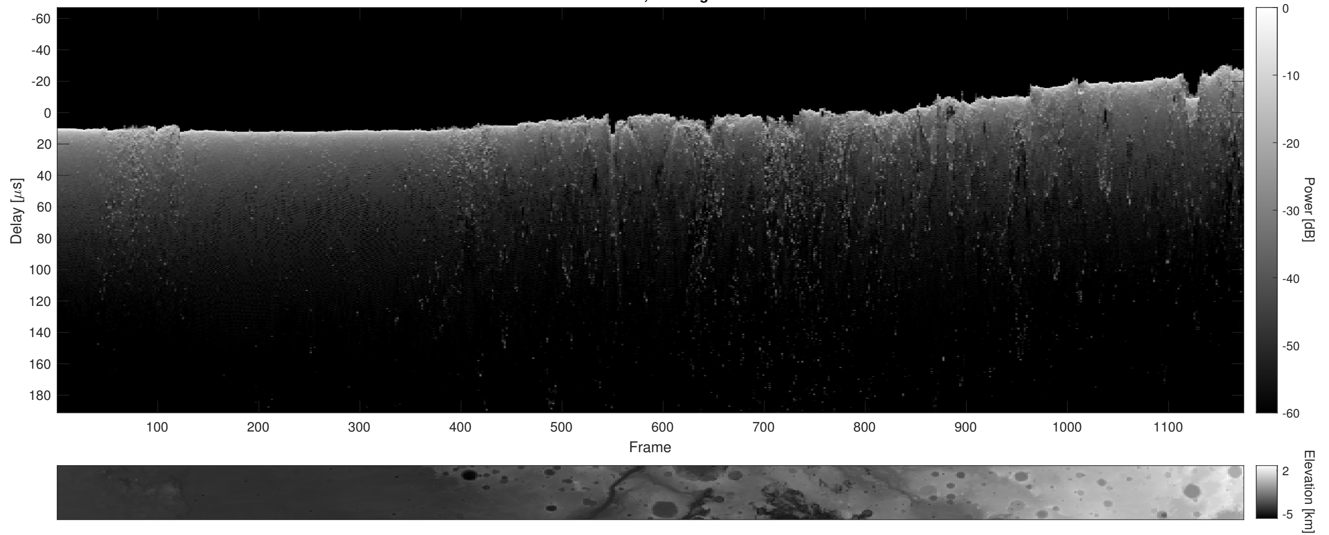
Orbit 17674, Cluttergram
