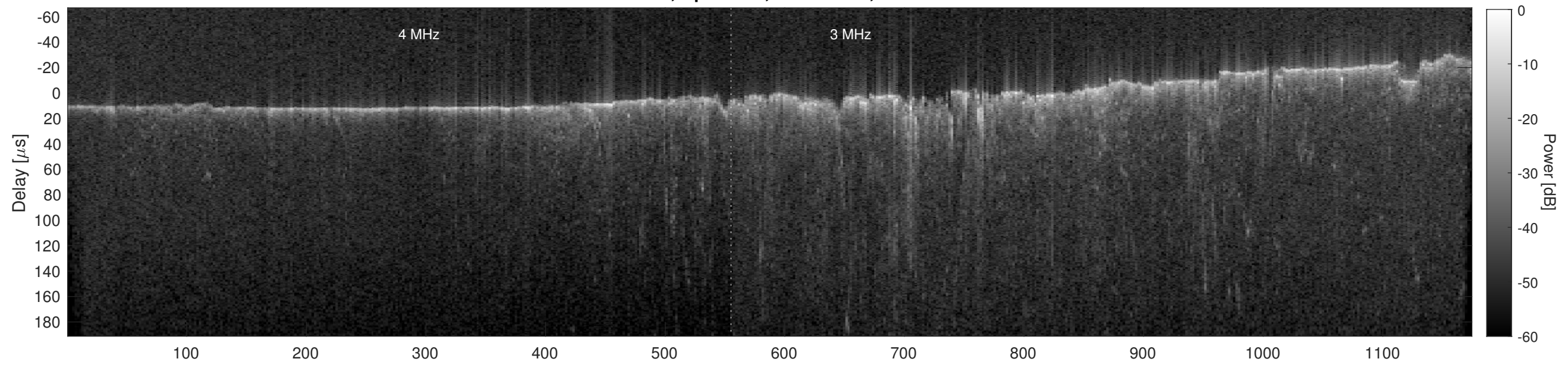
Orbit 17674, Cluttergram
