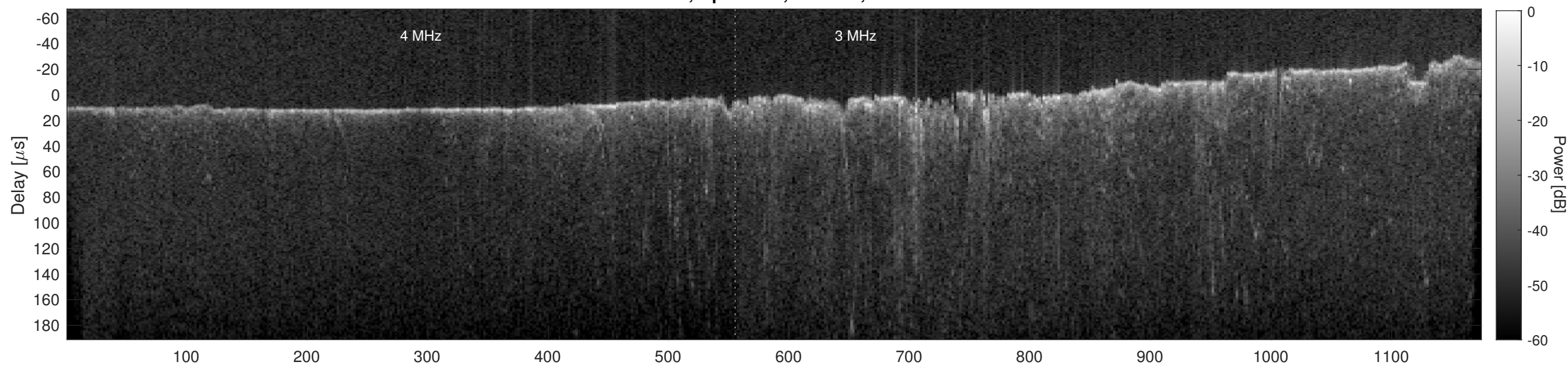
Orbit 17674, Cluttergram
