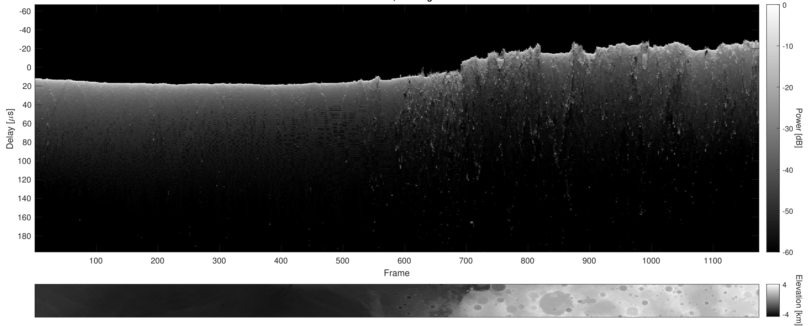
Orbit 17676, Cluttergram
