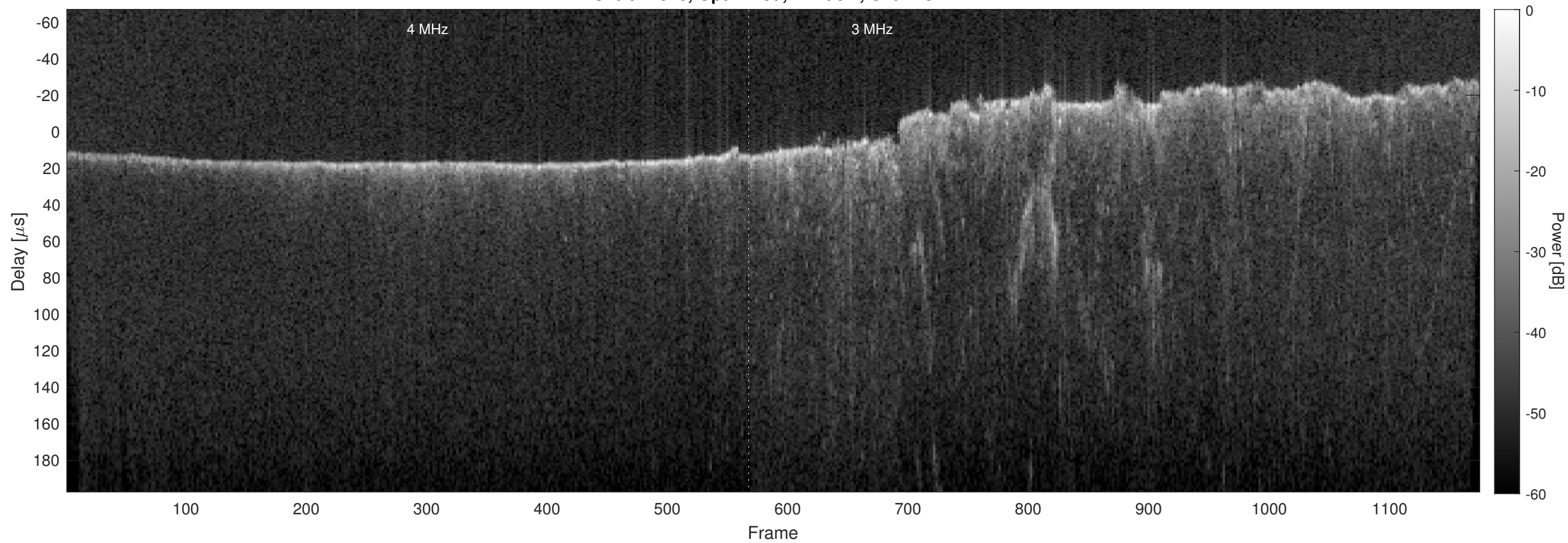
Orbit 17676, Optimized, Window, Channel 2
