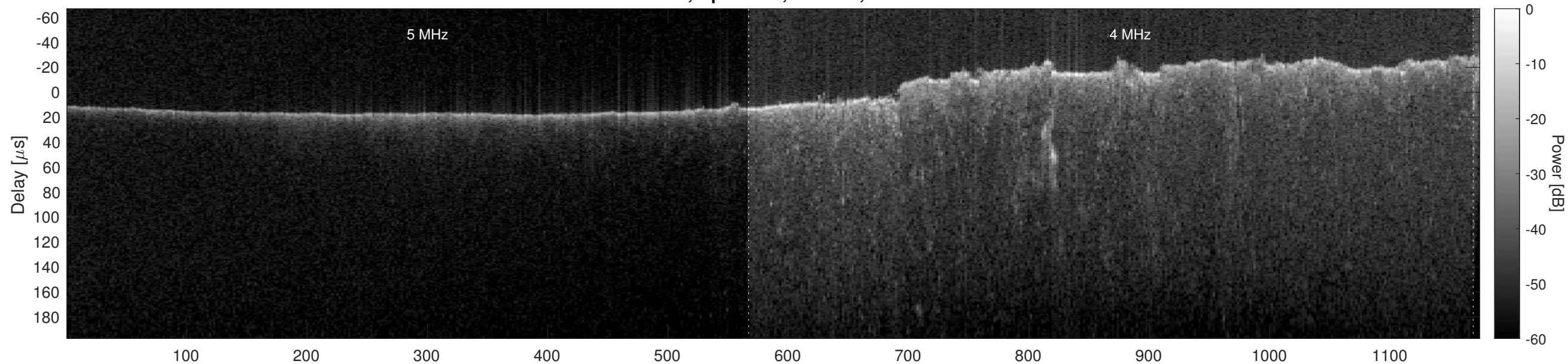
Orbit 17676, Optimized, Window, Channel 2
