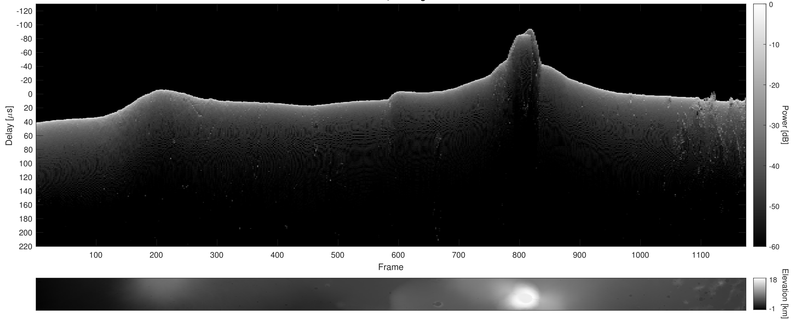
Orbit 17689, Cluttergram
