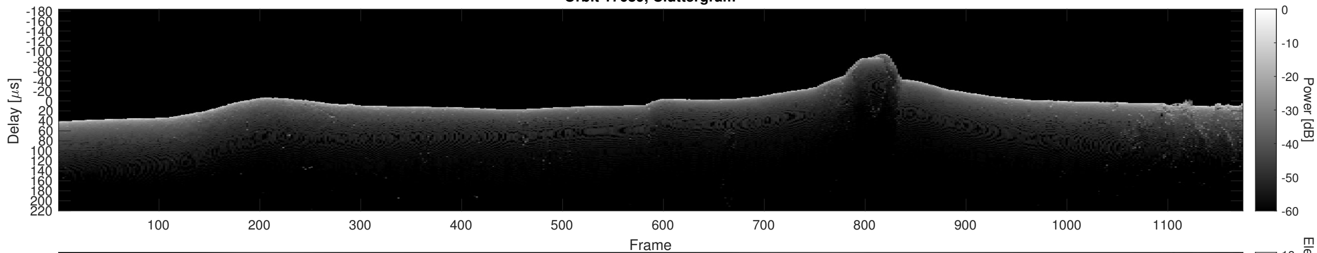
Orbit 17689, Cluttergram
