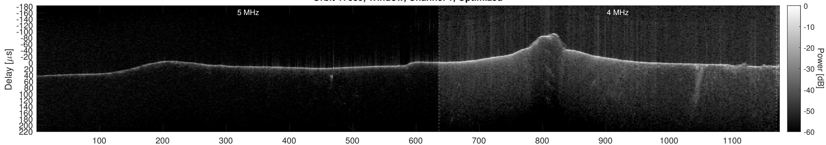
Orbit 17689, Cluttergram
