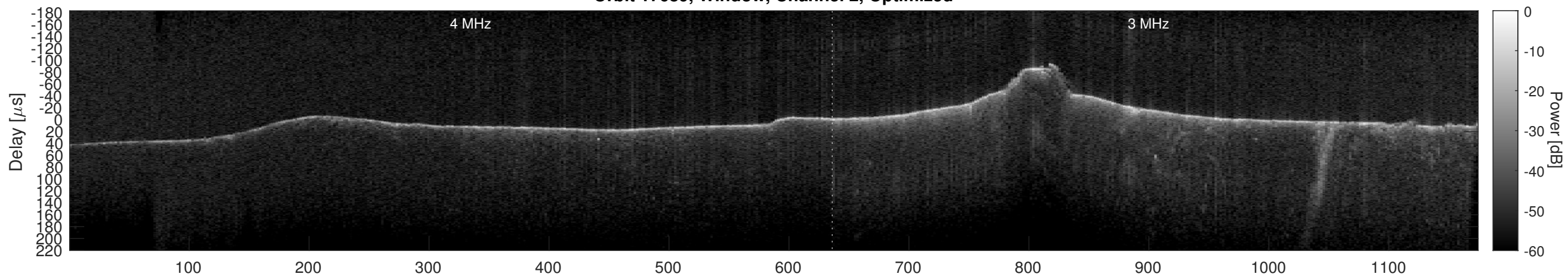
Orbit 17689, Cluttergram
