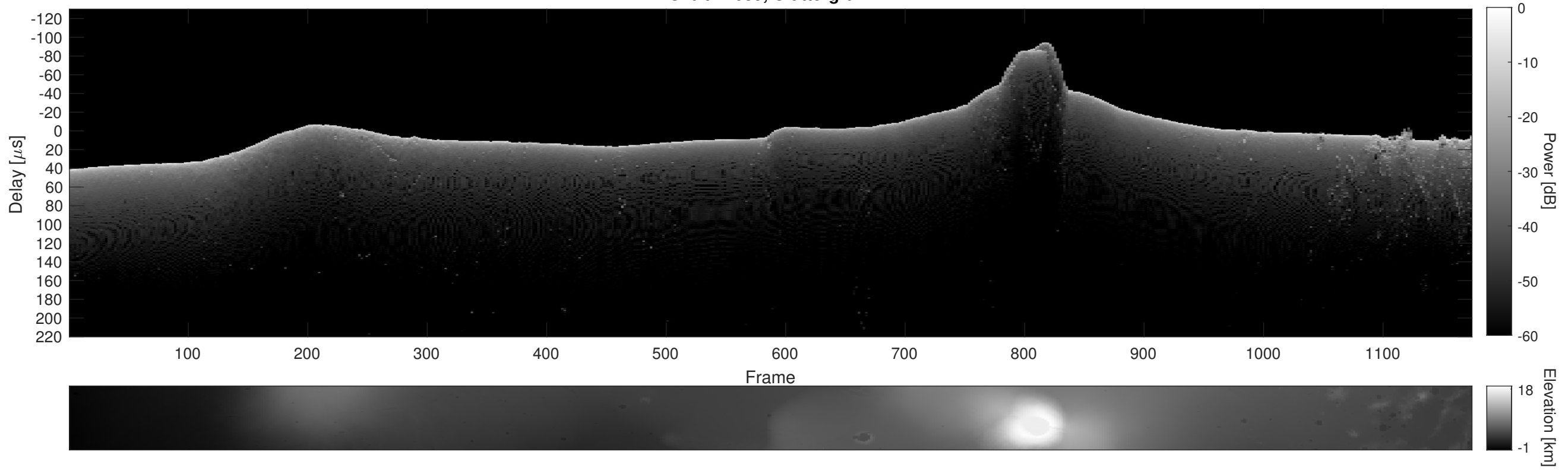
Orbit 17689, Cluttergram
