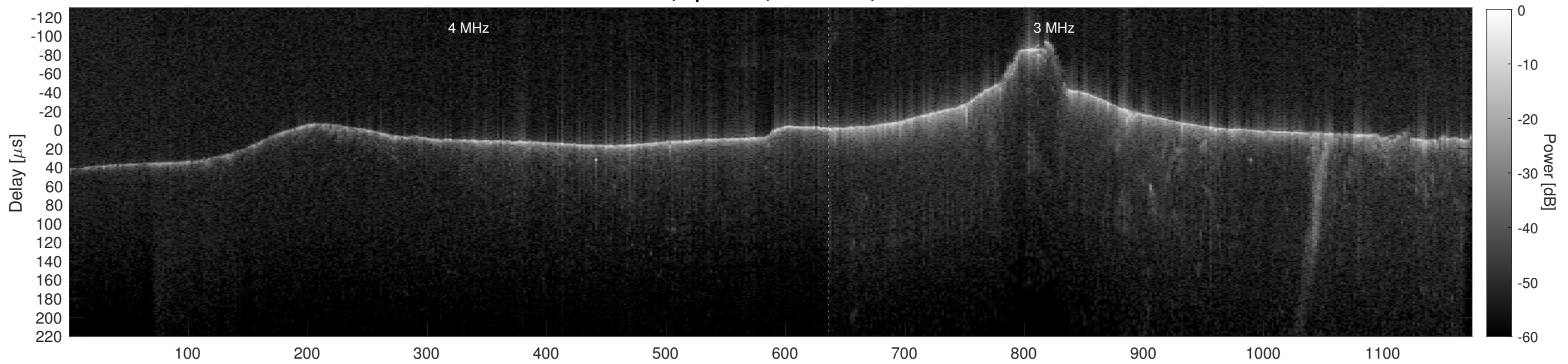
Orbit 17689, Cluttergram
