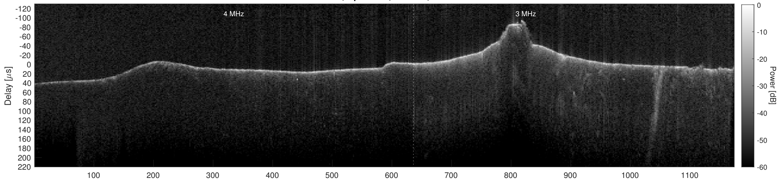
Orbit 17689, Cluttergram
