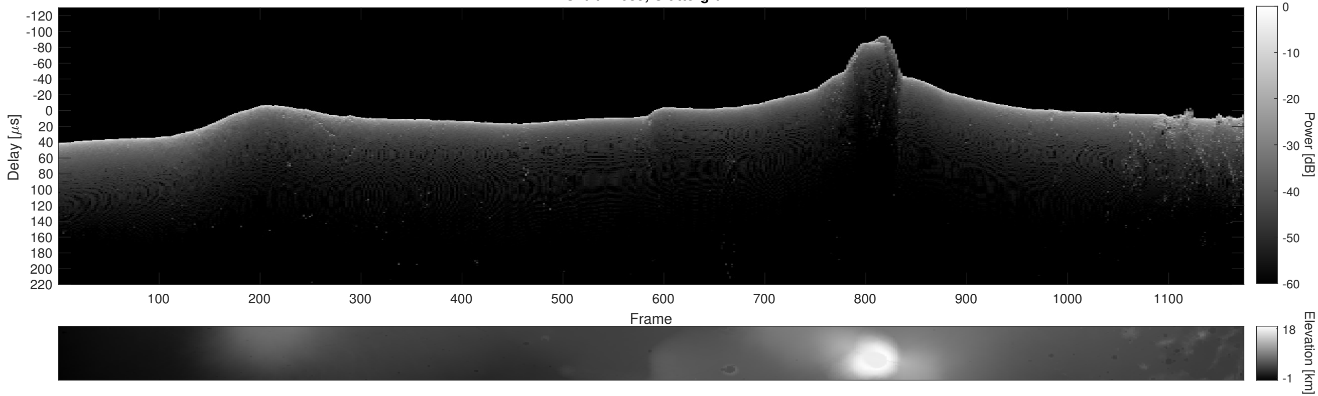
Orbit 17689, Cluttergram
